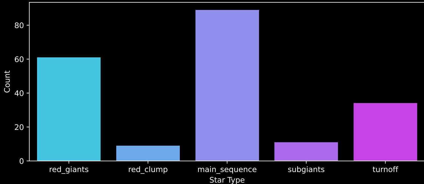
APOGEE DR17 Field: [CVZTILE_092+39_btx] Count plot of Star Type
