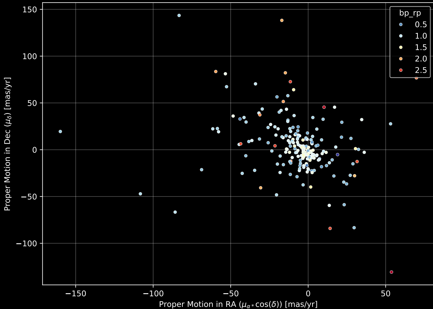
APOGEE DR17 Field: [CVZTILE_092+39_btx] Proper Motion Diagram (n= 204)
