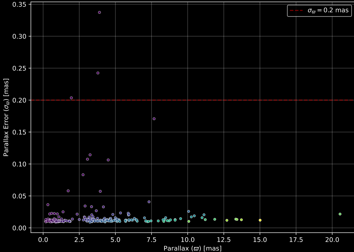
APOGEE DR17 Field: [CVZTILE_092+39_btx] Parallax Quality (n= 204)
