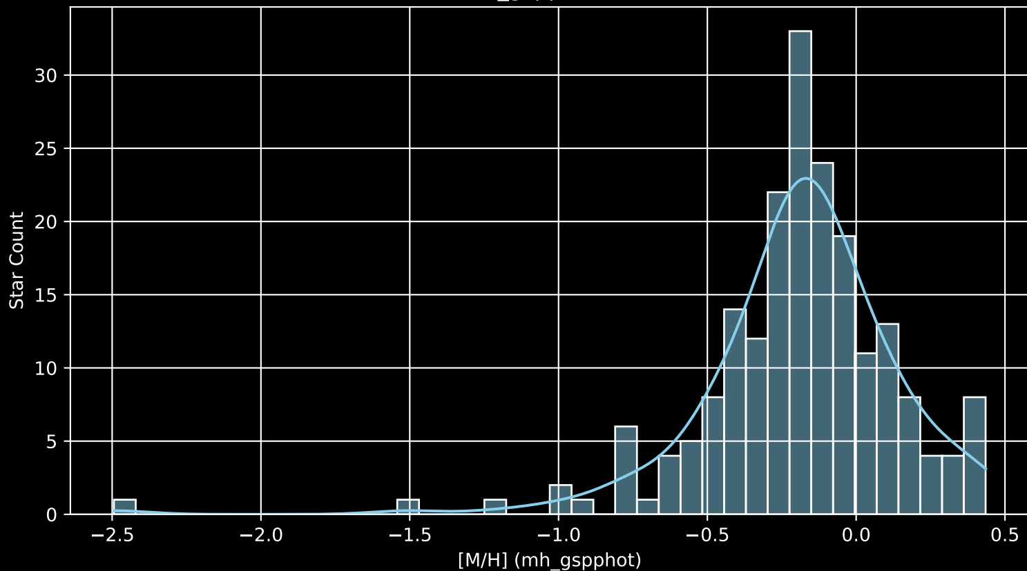
APOGEE DR17 Field: [CVZTILE_092+39_btx [M/H] (mh_gspphot) (n= 202)
