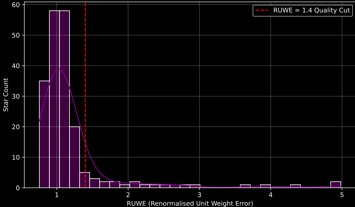
GAPOGEE DR17 Field [CVZTILE_092+39_btx] RUWE Distribution (n= 197)
